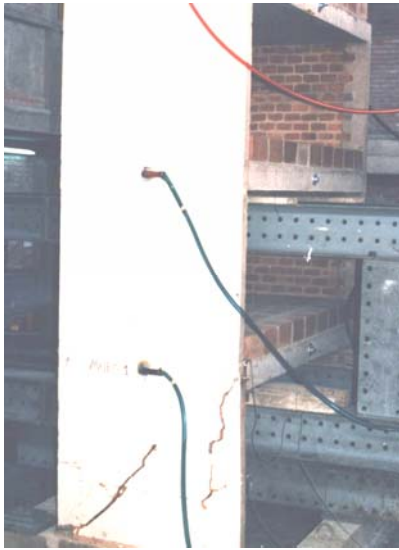
Fig. 5 Specimen after run C
