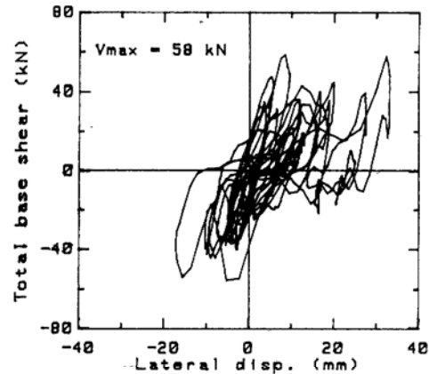
Fig. 8 Total base shear force vs. displacement at level 1 in run C
