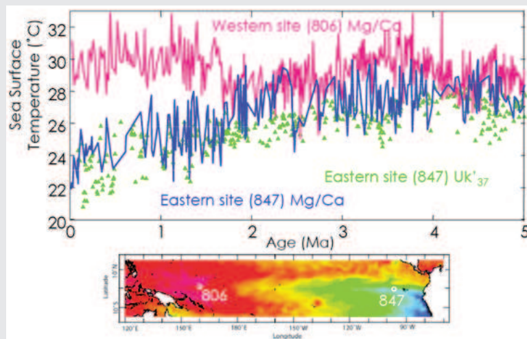
FIGURE 2.6 Changes in equatorial sea surface temperature gradients over time. The top panel shows time series of paleo-sea surface temperatures reconstructed for the western equatorial Pacific (ODP Site 806) using foraminiferal Mg/Ca ratio measurements of Globigerinoides sacculifer , and for the eastern equatorial Pacific (ODP Site 847) using Mg/Ca ratios of G. sacculifer as well as the biomarker U^{k'}_{37} index. Note the reduced sea surface gradient from 5 to 3 Ma, a gradual diversion of the records after that time, and a relatively strong gradient established after about 1.7 Ma. For comparison, the lower panel shows the present-day equatorial sea surface temperature gradient and the location of the eastern (Site 847) and western (Site 806) deep-sea coring sites.
