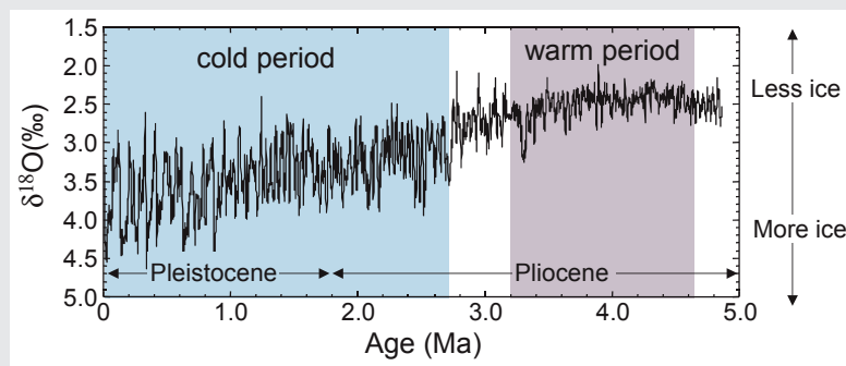
FIGURE 2.5 Benthic foraminifer \delta^{18}\text{O} record of high-latitude climate (primarily ice volume) from Ocean Drilling Program (ODP) cores, showing the relative warmth during the early Pliocene, followed by the transition into the cooler later Pliocene and Pleistocene.
