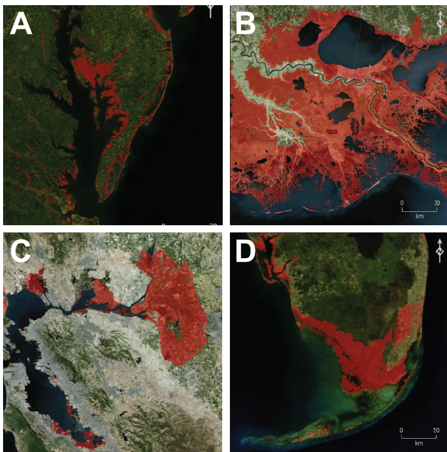
FIGURE 2.7 Effects of a 1-m rise in sea level (inundated areas with connectivity to the sea shown in red; see Weiss et al., 2011)—in the absence of human intercession—for four areas of the U.S. coastline: (A) Chesapeake Bay area; (B) New Orleans area; (C) San Francisco Bay area, and (D) South Florida. Because of the time needed for atmospheric \text{CO}_2 and surface warming to reach equilibrium, this amount of sea level rise might be anticipated even if anthropogenic sources of \text{CO}_2 were to cease today. In addition to local effects, inundation of the San Francisco Bay area and south Florida would have substantial impacts on water resources in both California and Florida.
