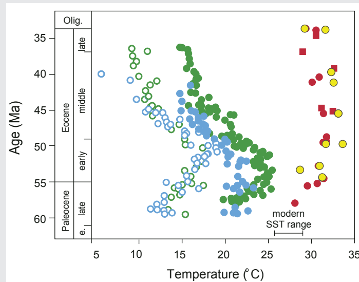
FIGURE 4.5 Tropical paleotemperature estimates based on \delta^{18}\text{O} data from unaltered benthic and planktonic foraminifera (red circles and squares, respectively) and from \text{TEX}_{86} data (yellow circles) from onshore drill core samples from Tanzania. These are plotted for comparison with benthic (open circles) and planktonic (green circles) foraminifera \delta^{18}\text{O} data from ODP cores collected from the tropical Pacific Ocean, inferred to have been diagenetically altered and thereby indicating anomalously low paleotemperature estimates. SOURCE: Pearson et al. (2007).
