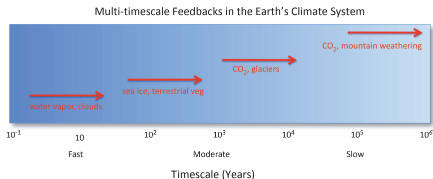
FIGURE 4.4 Schematic representation of the range of feedback scales that act on Earth's climate system.
