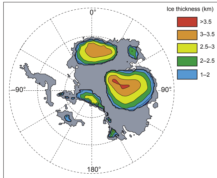
FIGURE 2.8 Modeled distribution of greenhouse ice sheets on Antarctica. Relatively small (~25 m) fluctuations in sea level have been associated with Antarctic ice (Galeotti et al., 2009), which would likely have built up in areas of high topography or near coastal moisture. SOURCE: DeConto and Pollard (2003), reprinted by permission of Macmillan Publishers Ltd.
