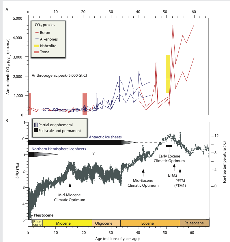
FIGURE 3.2 Relationship between atmospheric CO 2 (A) and climate (B) through the Cenozoic. The upper panel shows reconstructed p\text{CO}_2 from marine and lacustrine proxy records; the dashed line is maximum p\text{CO}_2 for the Neogene estimated by equilibrium calculations using lacustrine mineral phases (Lowenstein and Demicco, 2006). The climate curve in the lower panel is a composite of deep-sea benthic foraminiferal oxygen-isotope records, smoothed using a five-point running mean (Zachos et al., 2001a, 2008). The temperature scale on the right axis was calculated for an “ice-free ocean,” and is thus applicable solely to the pre-Oligocene portion of record.
