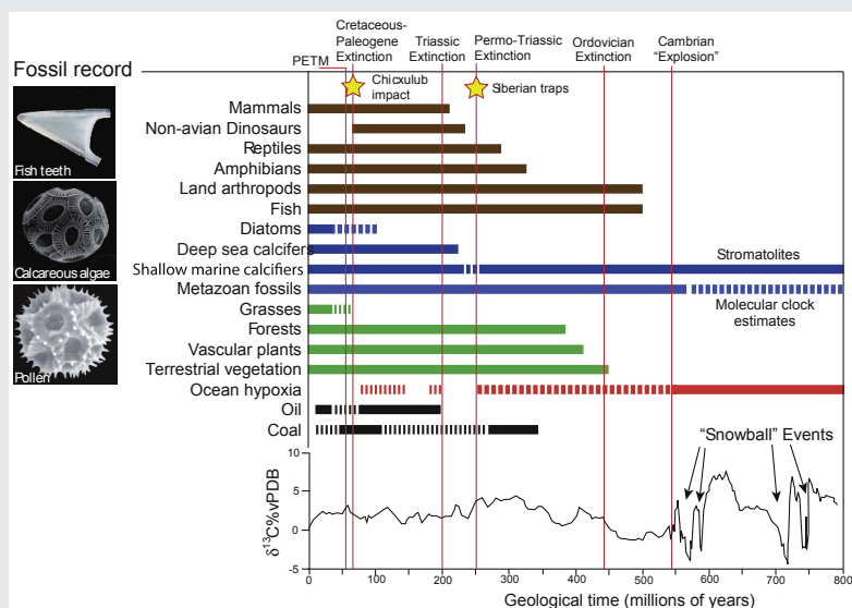
FIGURE 1.3 Timing of major events in late Precambrian and Phanerozoic evolution. From bottom to top: record of the carbon cycle from carbon isotopes, showing the transition from the high-amplitude cycles of the late Neoproterozoic—including several “snowball Earth” episodes—to the much more muted trends of the Phanerozoic (Hayes et al., 1999). Periods of abundant coal and oil formation, which include the extensive coal units of the Carboniferous and Permian, Cretaceous coal, and extensive coal deposits of the Paleogene Arctic, as well as oil deposits formed during Jurassic and Cretaceous oceanic anoxic events and Mio-Pliocene oil deposits of the Pacific Rim (Windley, 1995), are shown in black. Ocean hypoxia (red line) illustrates the reduction in the extent of anoxic or hypoxic conditions in the deep sea with time, with low oxygen common in the Paleozoic and intermittent episodes of basinwide to global oceanic anoxic events in the Mesozoic. The extent of vegetation cover is shown with green lines, and major groups of oceanic organisms that contribute to global geochemical cycles either through burrowing (metazoans; Sheehan, 2001), marine calcifiers that buffer ocean pH (Ridgwell et al., 2003), or diatoms with their role in the silica cycle (Ridgwell et al., 2002; Cortese et al., 2004; Lazarus et al., 2009), are shown in blue. Fish (brown line) appear in the early Cambrian (Shu, 1999) and give rise to terrestrial amphibians in the Devonian (Selden, 2001). The invasion of land is accomplished by terrestrial arthropods well before the appearance of terrestrial vertebrates. Non-avian dinosaurs and mammals evolved from reptiles in the early Mesozoic (Sereno, 1999; Brusatte et al., 2008). Reptiles show multiple invasions of the oceans in the Mesozoic, and mammalian groups invade the ocean several times in the Cenozoic.
