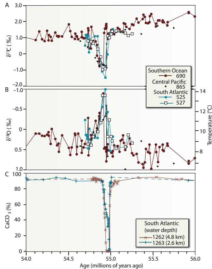
FIGURE 3.3 Marine stable isotope and seafloor sediment \text{CaCO}_3 records compiled using several ocean drilling sites for the PETM, a hyperthermal with some parallels to modern greenhouse gas-driven global change. (A) \delta^{13}\text{C} time series developed from benthic foraminifera illustrating ~2.5 part per thousand (‰) excursion at ~55 Ma. (B) \delta^{18}\text{O} time series and inferred temperatures record the prolonged period of ocean warming (~70–80 ky) and its large magnitude. There may have been several events of greenhouse gas release during the PETM that produced the large, abrupt changes in ocean temperatures. (C) Record of seafloor calcium carbonate content from the South Atlantic documents the significant reduction due to dissolution and deep-ocean acidification during the PETM. The apparent onset of \text{CaCO}_3 dissolution prior to the onset of the carbon isotope excursion reflects the extensive dissolution of uppermost Paleocene sediments by acidic waters during the PETM.
