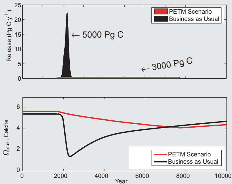
FIGURE 3.4 Initial carbon pulse for the PETM (red curves), estimated to be 3,000 Pg carbon using published carbon isotope and observed deep-sea carbonate dissolution records, and a carbon cycle model (LOSCAR; Zeebe et al., 2008, 2009). The magnitude of the input carbon mass was inferred from carbonate dissolution records, with the \delta^{13}\text{C} of the carbon pulse ( \leq -50\text{‰} ) constrained by requiring the model outcome to match observed deep-sea \delta^{13}\text{C} records. The model assumes a large initial input of carbon over 5 ky, followed by further smaller pulses and a low continuous carbon release (an additional 1,500 Pg) throughout the PETM main event. Changes in calcite saturation in the surface ocean (lower diagram) are estimated for the PETM (red curve) and for the future (black curve), based on the inferred magnitude of the carbon pulse to atmosphere. SOURCE: Courtesy of R.E. Zeebe, personal communication (2010).
