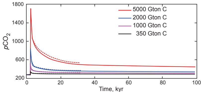
FIGURE 3.6 Schematic showing the predicted long-term response over 100,000 years of atmospheric \text{CO}_2 , including ocean temperature feedbacks, to a range of possible fossil fuel emissions totals. The 100,000-year simulations include silicate weathering (solid lines) and the 35,000-year simulations include seafloor \text{CaCO}_3 dissolution (dashed lines). These models highlight how the timescale of carbon uptake becomes extended as the event unfolds. Fast processes such as ocean uptake and biomass growth, with high transfer rates but limited capacity, lose their potency, while slower processes, such as seafloor carbonate dissolution and rock weathering, come to dominate.
