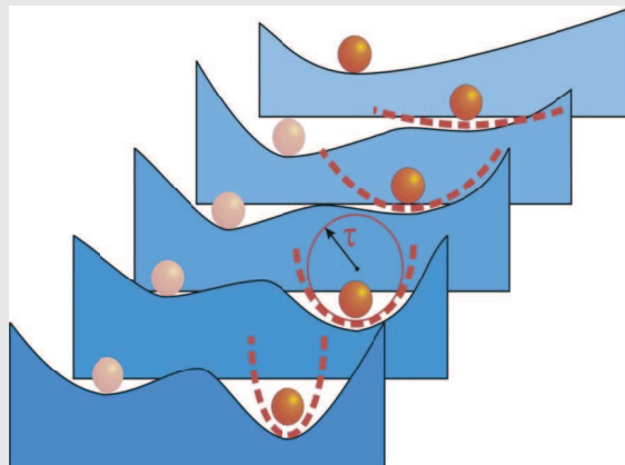
FIGURE 3.1 Equilibrium states of a “system” (valleys) in response to gradual anthropogenic CO 2 forcing (progressing from dark to light blue). The curvature of the valley is inversely proportional to the system’s response time ( \tau ) to small perturbations. A threshold is reached when the valley becomes shallower and finally vanishes causing the ball to abruptly roll to a new state (to the left).
