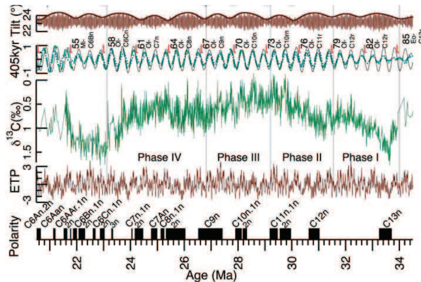
FIGURE 4.2 Astronomically tuned climate record from the Oligocene of the Central Pacific. Top two panels show the astronomical calculation of the 41,000-year cycle in the tilt of Earth's spin axis (known as obliquity), and the 100,000-year cycle in eccentricity (thin black line). In the middle panel is the carbon isotope record of the deep Pacific which displays a well developed ~400,000-year cycle that closely matches the calculated astronomical cycle (dashed green line). ETP is the calculated cycle expected if the sediment record integrated the combined eccentricity, tilt and precession cycles. The geomagnetic polarity timescale is shown on the bottom, here calibrated to the astronomical cycles.
