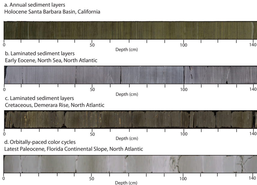
FIGURE 4.1 Sediment cores can be detailed recorders of time: (a) Core sample (Core MV1012-TC-3) from the Holocene of Santa Barbara Basin, California, displaying well-developed millimeter-scale laminations related to annual cycles in biological productivity and sediment runoff. (b) Eocene laminated sediments from the North Sea (Nini-3 well), potentially offering very high resolution records of climate and ecosystem variability. (c) Similar laminations in a drill core through Cretaceous black shales from the tropical North Atlantic (from ODP Site 1259). (d) Orbital cycles in sediment color paced by the precession cycle (~21 kyr) from a drill core in the Paleocene of the western North Atlantic (from ODP Site 1051; Norris and Röhl, 1999).
