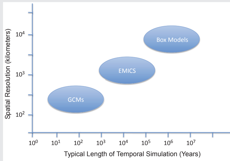
FIGURE 4.3 Graphical representation of the ranges of spatial resolution and simulation run times for the major categories of climate model.
