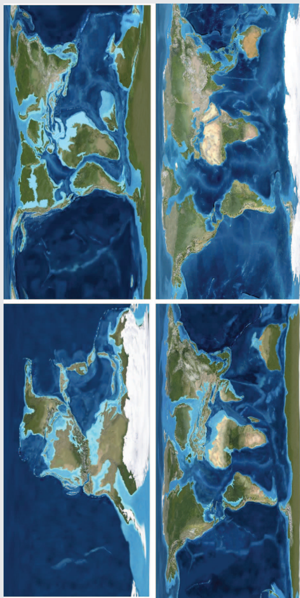
FIGURE 2.1 Continental configurations for the Pennsylvanian (upper left), mid-Cretaceous (upper right), Eocene (lower left), and mid-Pliocene (lower right). Topography was defined on the basis of digital elevation maps of modern Earth from the U.S. Geological Survey; colors portray climate and vegetation distribution based on a synthesis of all geological literature relevant to each time slice. SOURCE: Courtesy R.C. Blakey, Colorado Plateau Geosystems.
