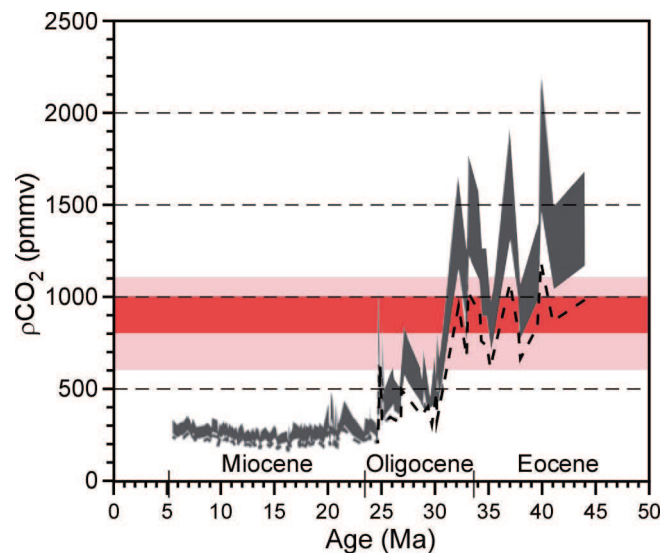
FIGURE 2.2 Estimated atmospheric p\text{CO}_2 for the past 45 million years (late Eocene through Miocene) calculated using all available stable carbon isotopic values of diunsaturated alkenones in deep-sea sediments. Values of \text{CO}_{2\text{aq}} were translated to atmospheric p\text{CO}_2 using Henry's Law and a range of dissolved phosphate values and sea surface temperatures for each site, and a salinity of 35 parts per thousand. The dark gray shaded region shows the range of maximum to intermediate estimates, and the dashed line represents minimum estimates. The uncertainty in p\text{CO}_2 estimates ranges from ~20 percent for the Miocene to 30 to 40 percent for the Paleogene. The broad pale red band ( p\text{CO}_2 values of 600-1,100 parts per million by volume) encompasses most of the \text{CO}_2 concentration range for nonmitigation emission scenarios projected for the end of this century (figure 10.26 in IPCC, 2007); the dark red band (values of 800-1,000 ppmv) corresponds to the Intergovernmental Panel on Climate Change (IPCC) A2 "business-as-usual" scenario. SOURCE: Modified after Pagani et al. (2005).
